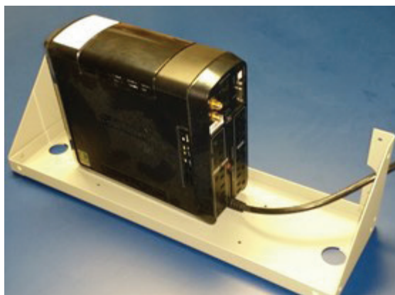
UPS with Mounting Shelf
